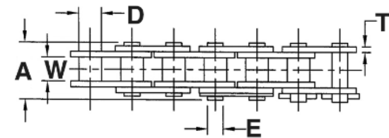
Fig.2 - Single Strand Roller Chain Drawing (Top View).
