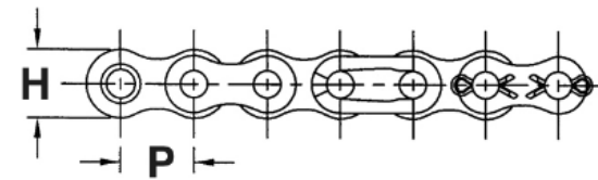
Fig.1 - Single Strand Roller Chain Drawing (Side View).
